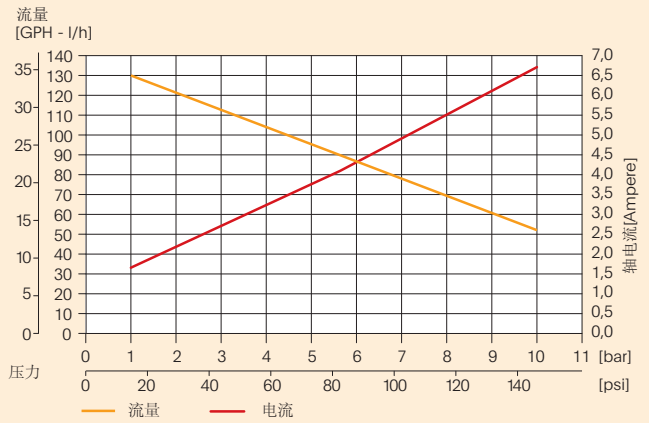
GA072-24V42x100mm无刷电机(90-93-02)
