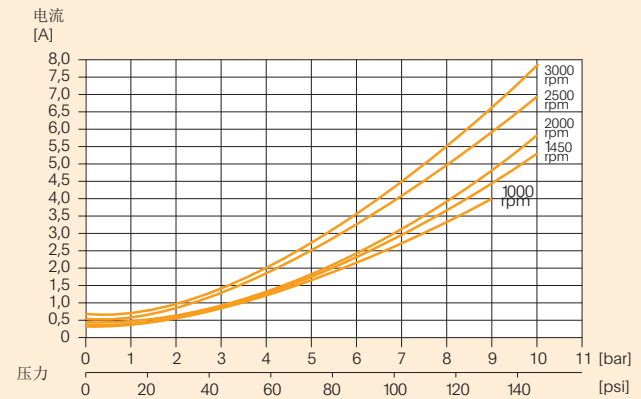
GA072-24V42x100mm无刷电机(90-93-02)
