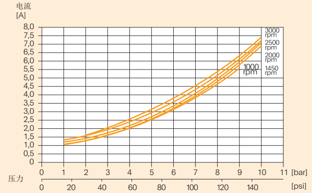
GA102-24V42x100mm无刷电机(90-93-02)
